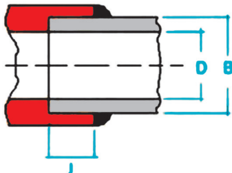
Fig. 5.22: Socket-welded joint
