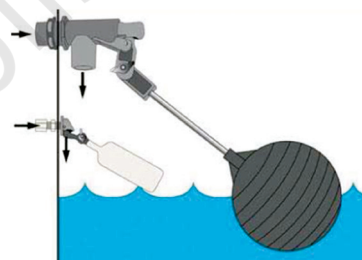
Fig. 5.44: Float valve
